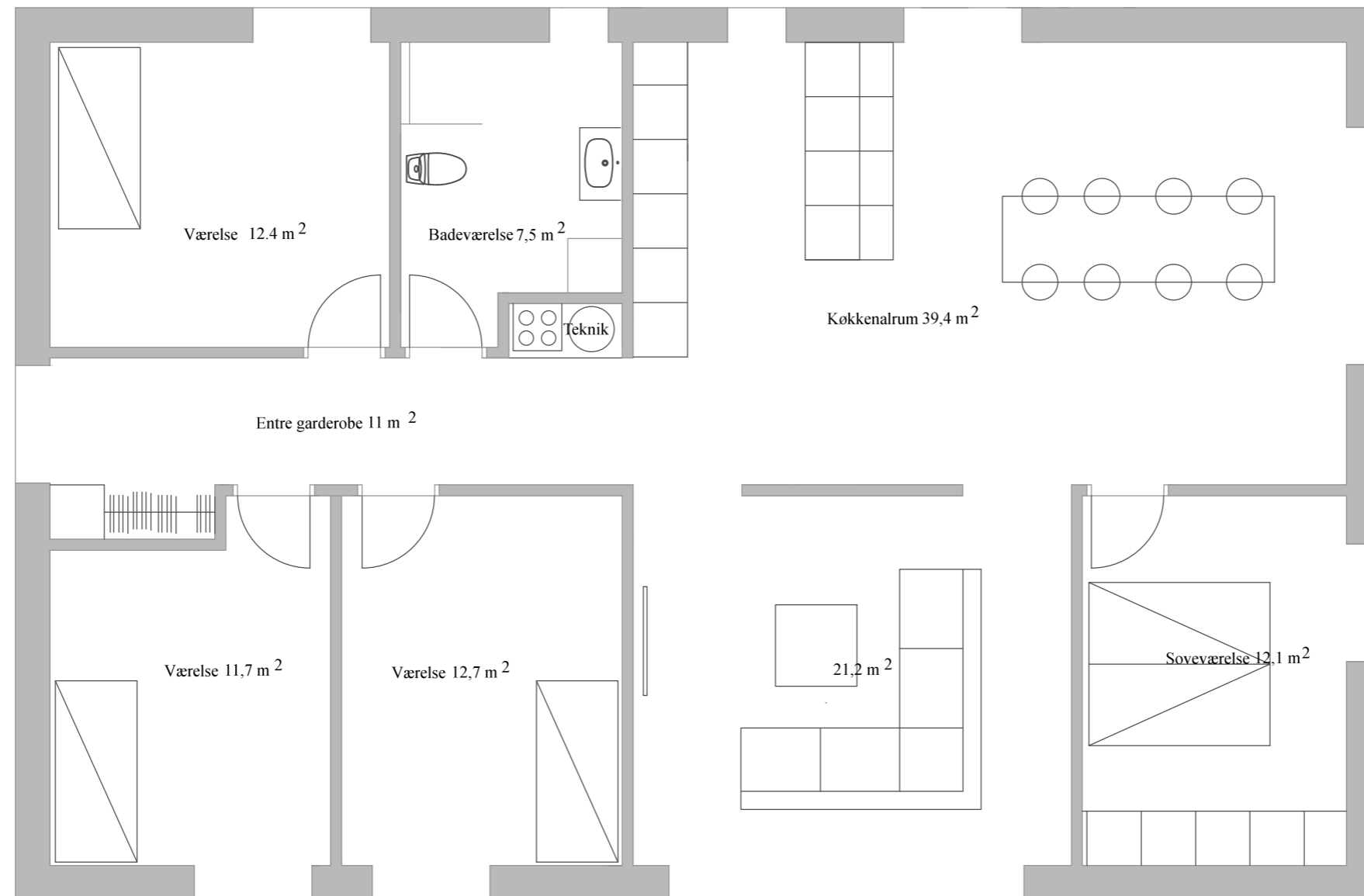
PLANTEGNING MODEL 148
